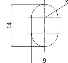
Mounting Hole
